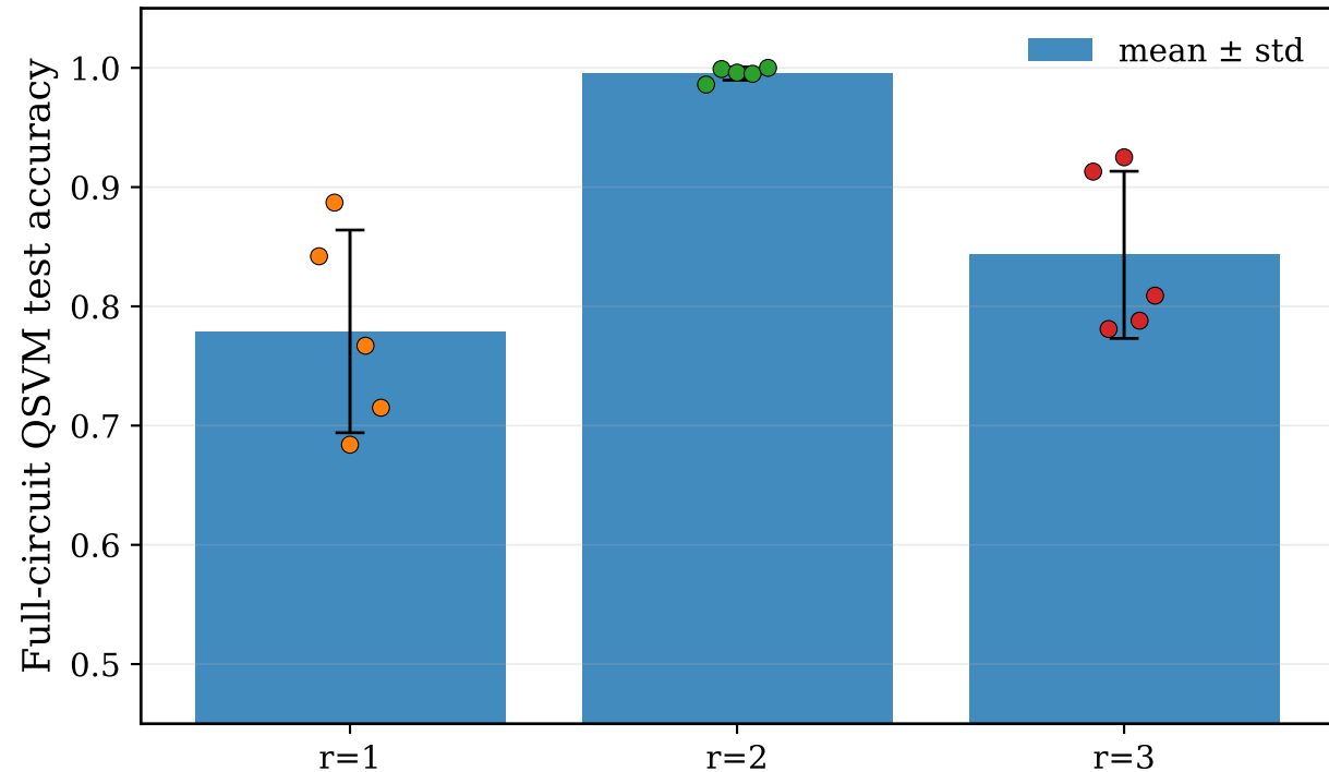
QSVM accuracy across five dataset splits
