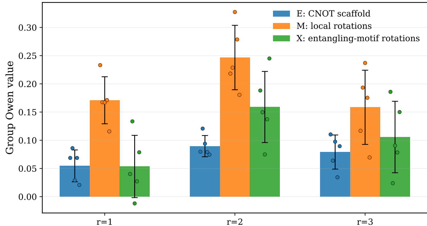
E/M/X group Owen values across five dataset splits
