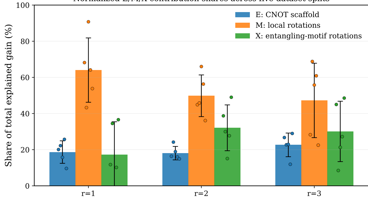
Normalized E/M/X contribution shares across five dataset splits
