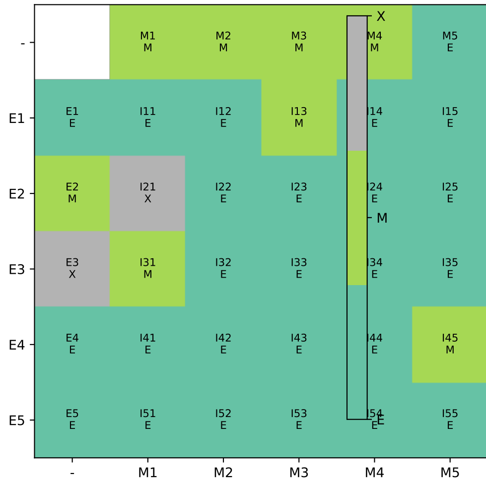
Top group for entanglement value
