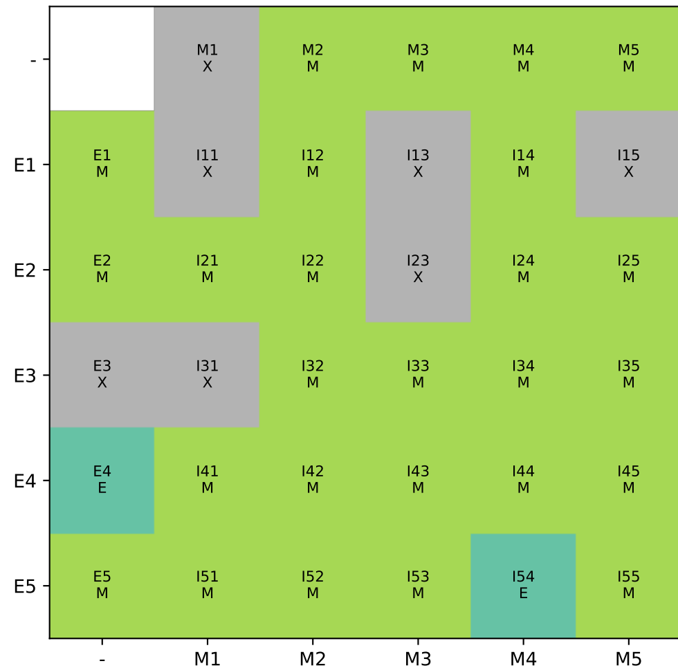
Top group for magic value
