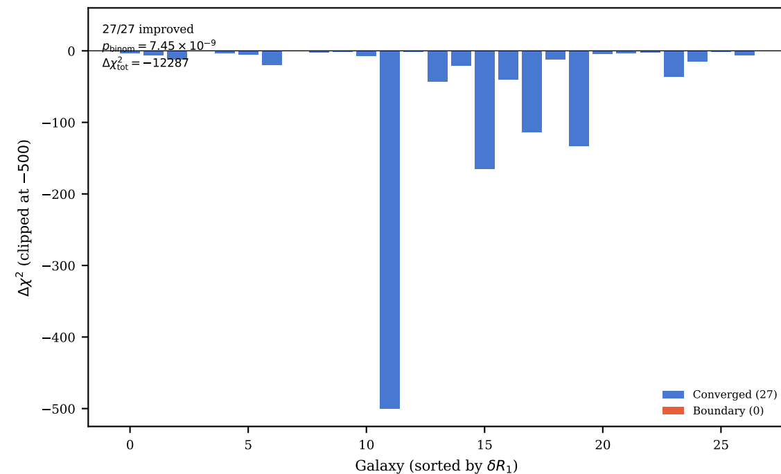
(e) Regime 2: c_{200}^{\text{BPB}} correction (27 virialized)
