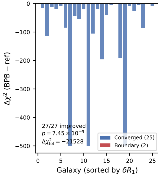
(b) \chi^2 improvement with c_{200}^{\text{BPB}}
