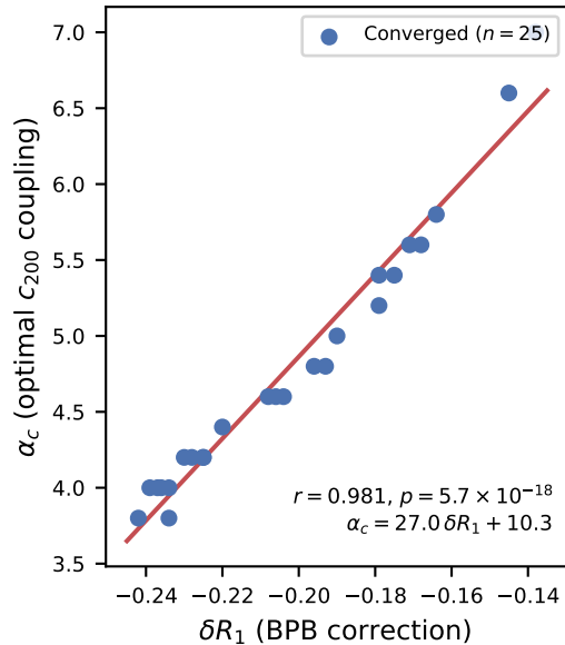
(c) \delta R_1 \rightarrow \alpha_c correlation
