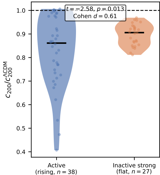
(a) Two-regime structure
