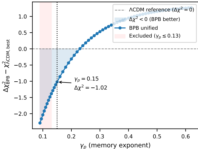
(a) \chi^2 landscape vs \gamma_p (KiDS-1000)
