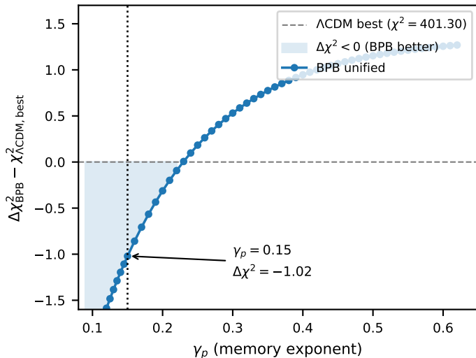
(a) \chi^2 landscape vs \gamma_p on KiDS-1000
