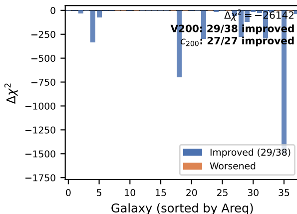
(b) \Delta\chi^2 per galaxy (38 active)
