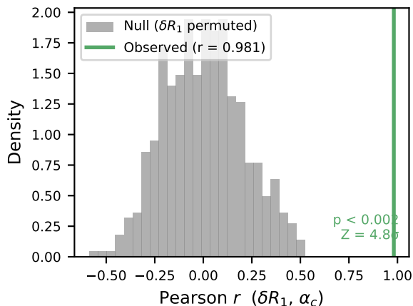
(a) Regime 2 null test ( \delta R_1 \rightarrow \alpha_c )
