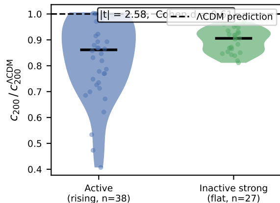
(c) Two physical regimes
