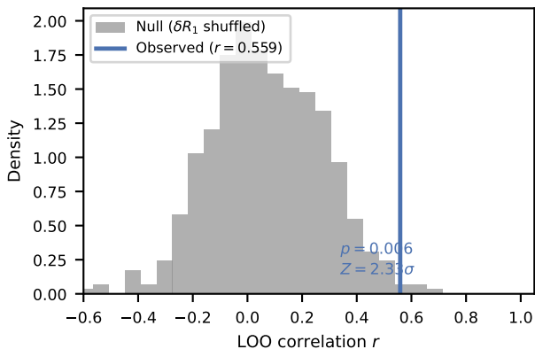
(a) Synthetic null test (500 perms)
