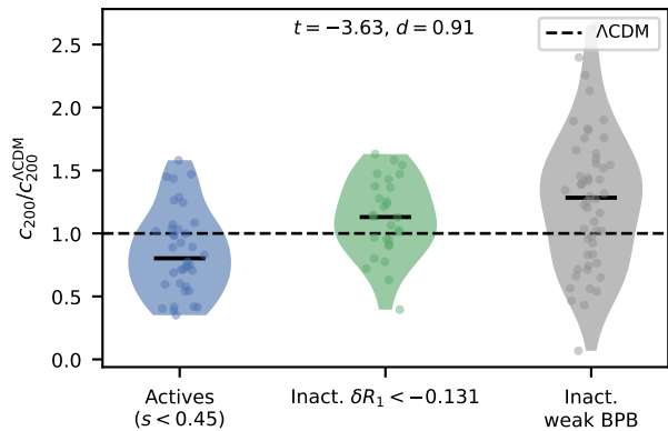
(c) Two physical regimes
