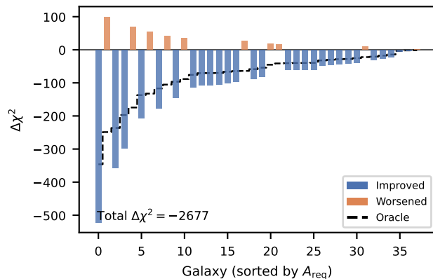
(b) \Delta\chi^2 per galaxy (38 actives)
