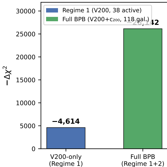
(b) \Delta\chi^2 summary (118 galaxies)
