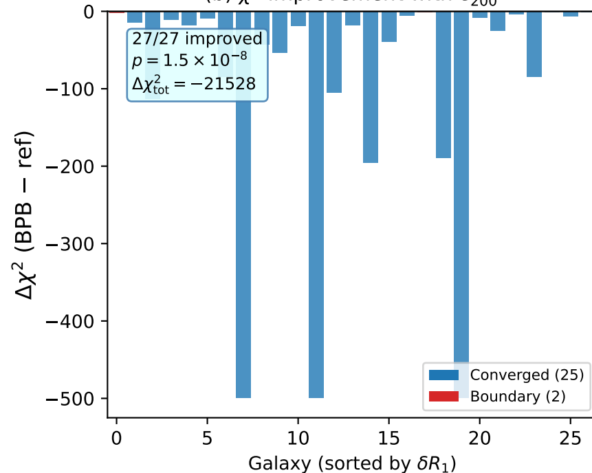
(b) \chi^2 improvement with c_{200}^{\text{BPB}}
