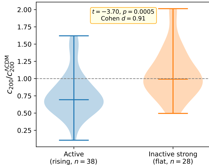
(a) Two-regime structure
