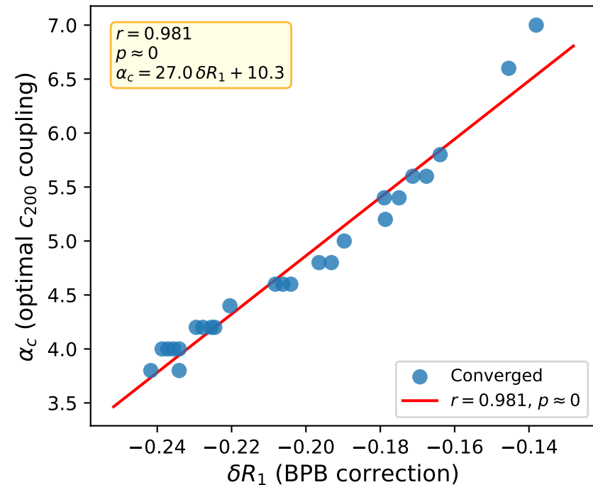
(c) \delta R_1 \rightarrow \alpha_c correlation
