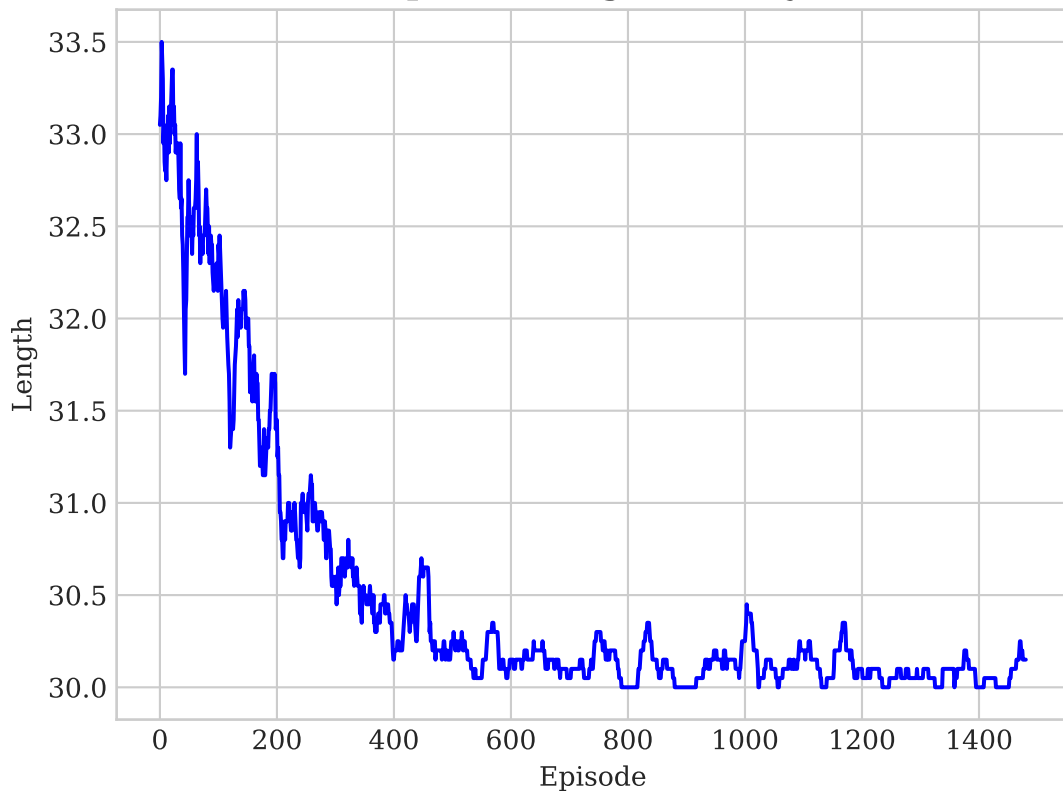
Episode Length - Policy
