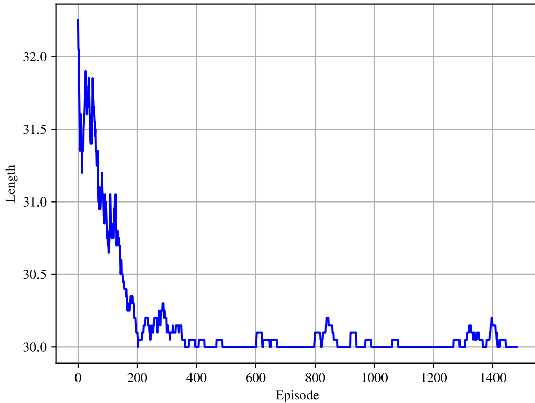
Episode Length - DeepQLearning
