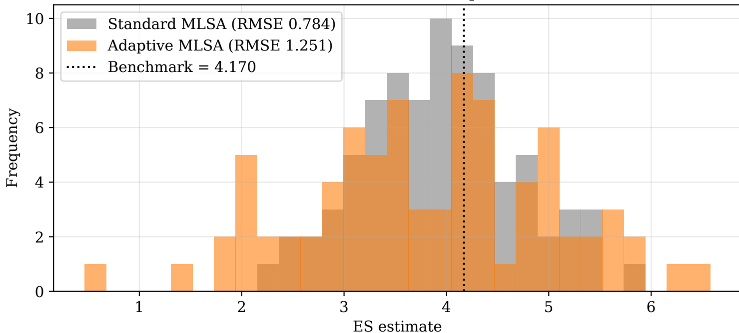
heston ES: standard vs adaptive MLSA
