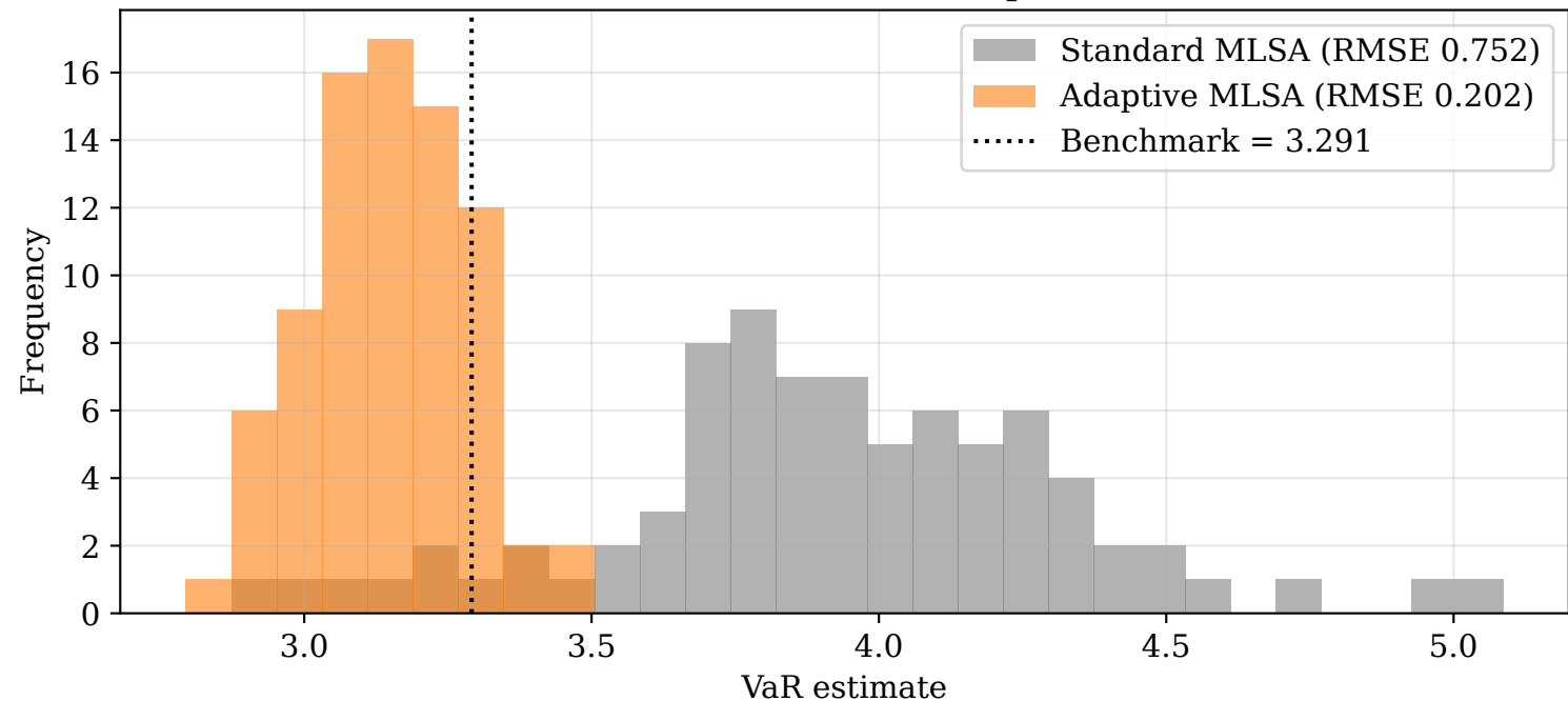
heston VaR: standard vs adaptive MLSA
