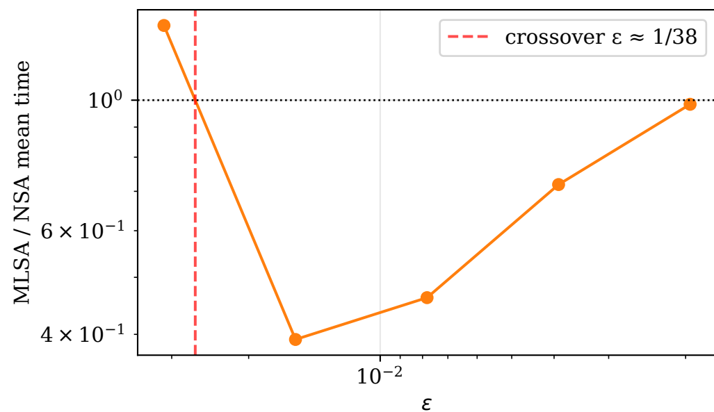
heston VaR
