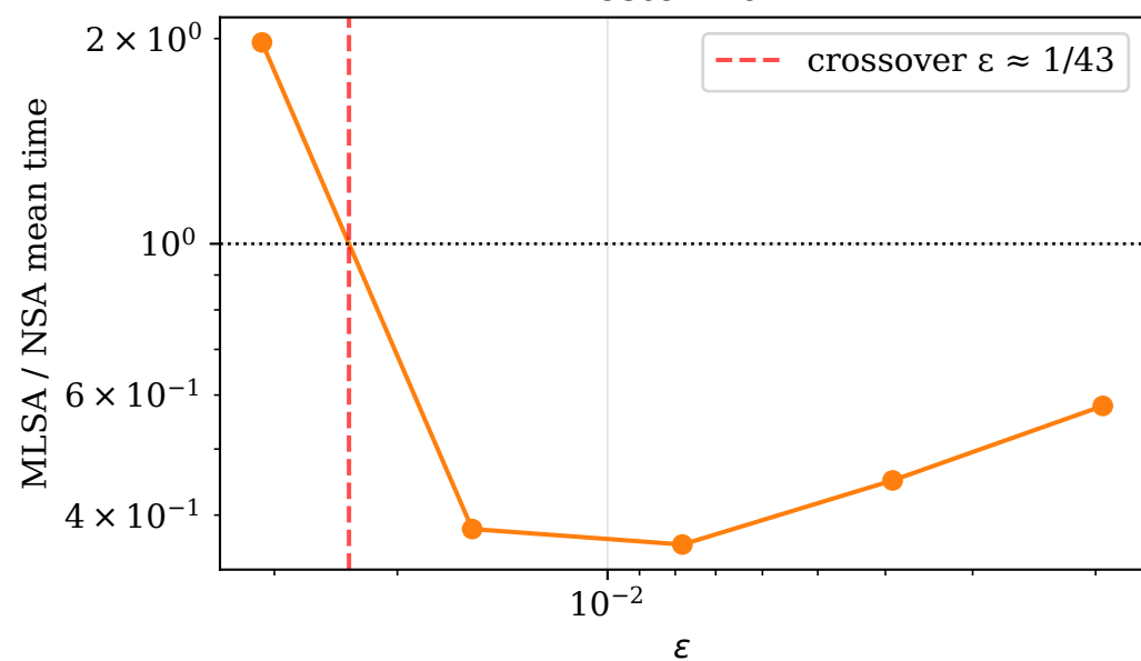
heston VaR
