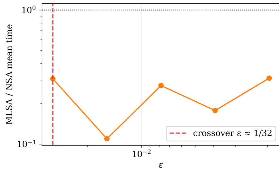
merton VaR
