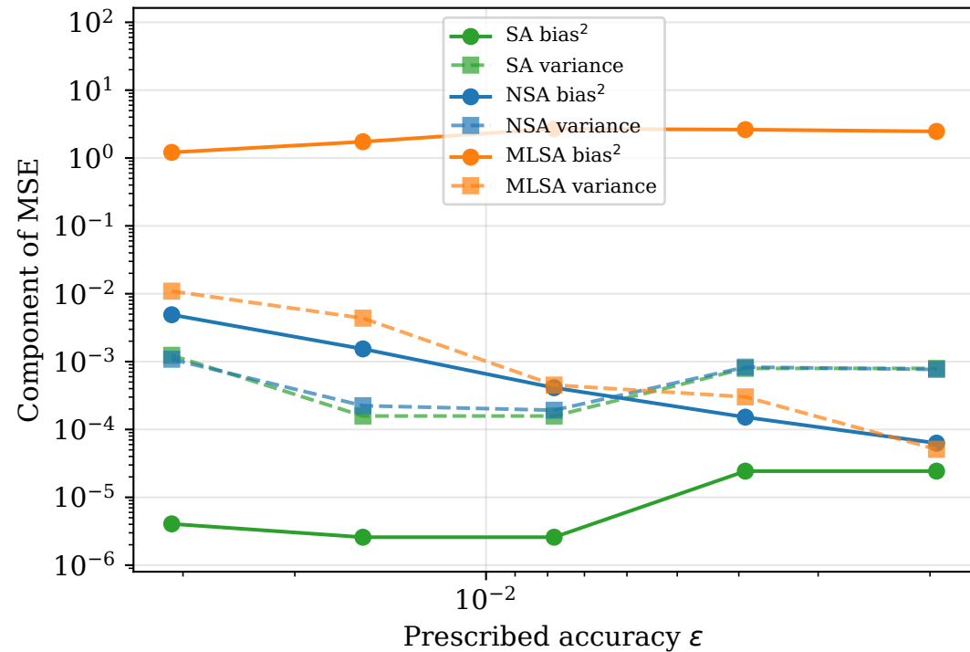
bs VaR: bias 2 vs variance
