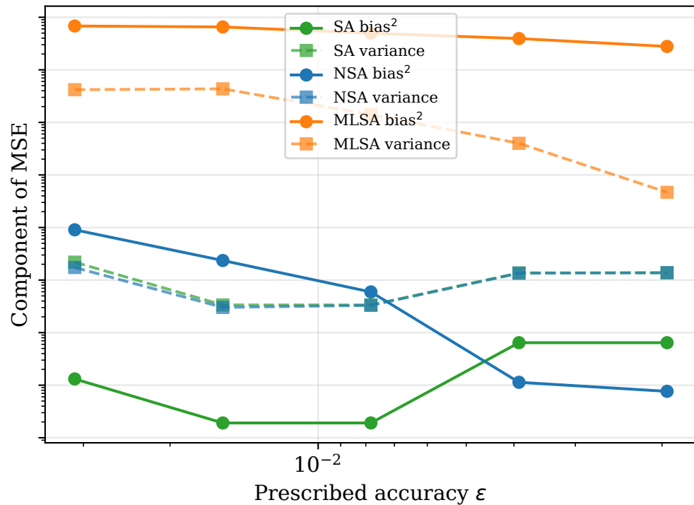
bs ES: bias 2 vs variance
