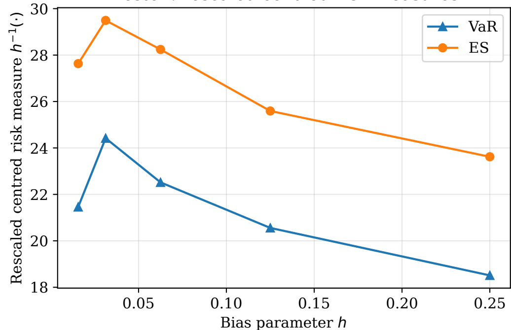
Heston: rescaled centred risk measures
