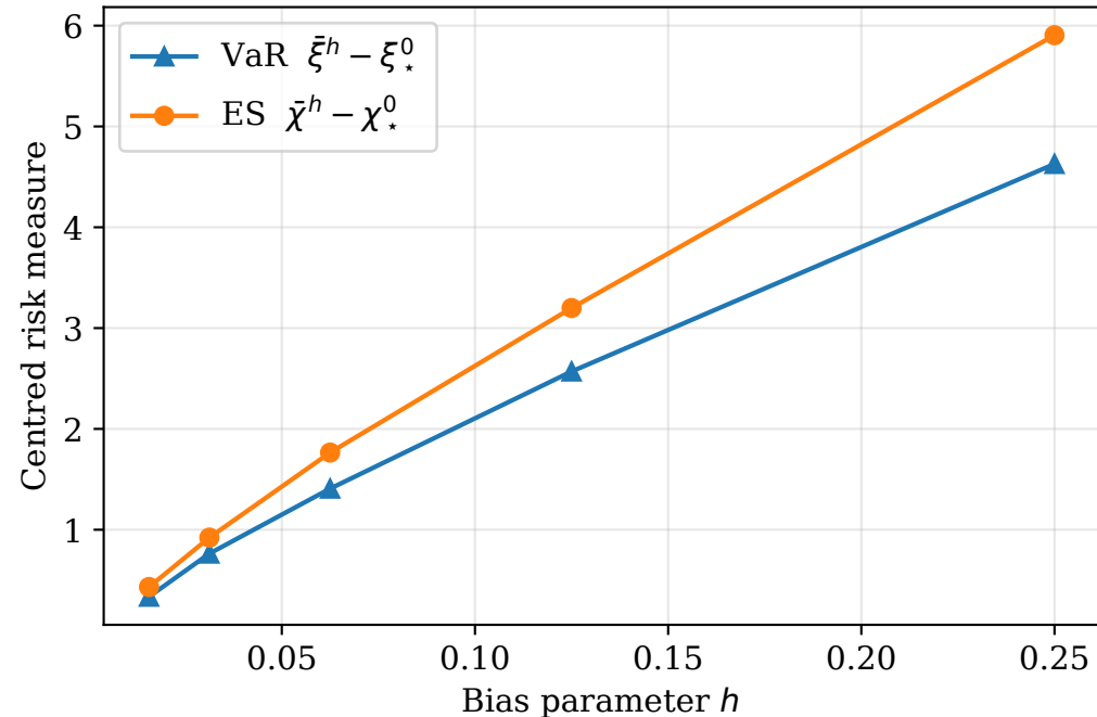
Heston: centred risk measures
