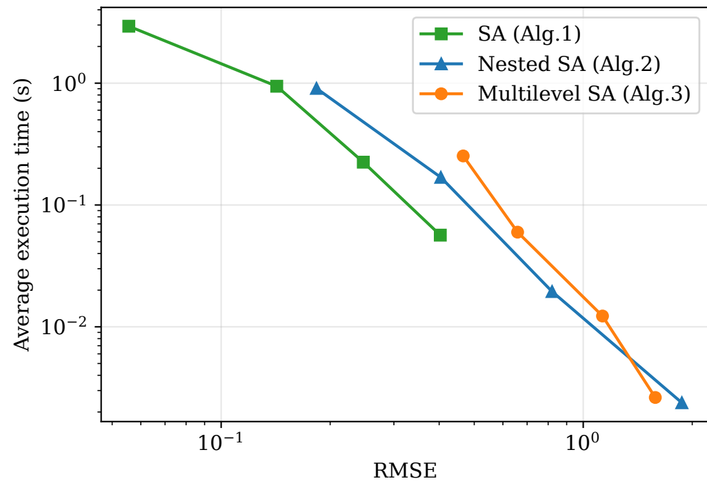
Heston VaR
