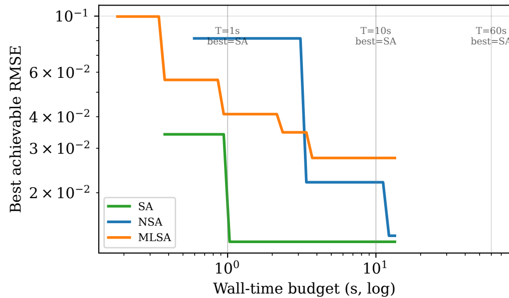
merton VaR
