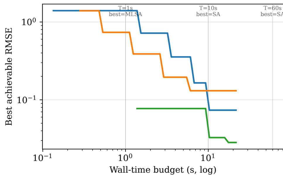
heston VaR
