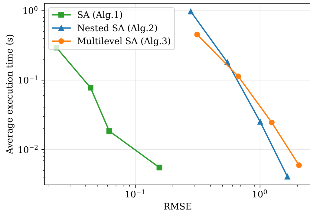
Merton VaR
