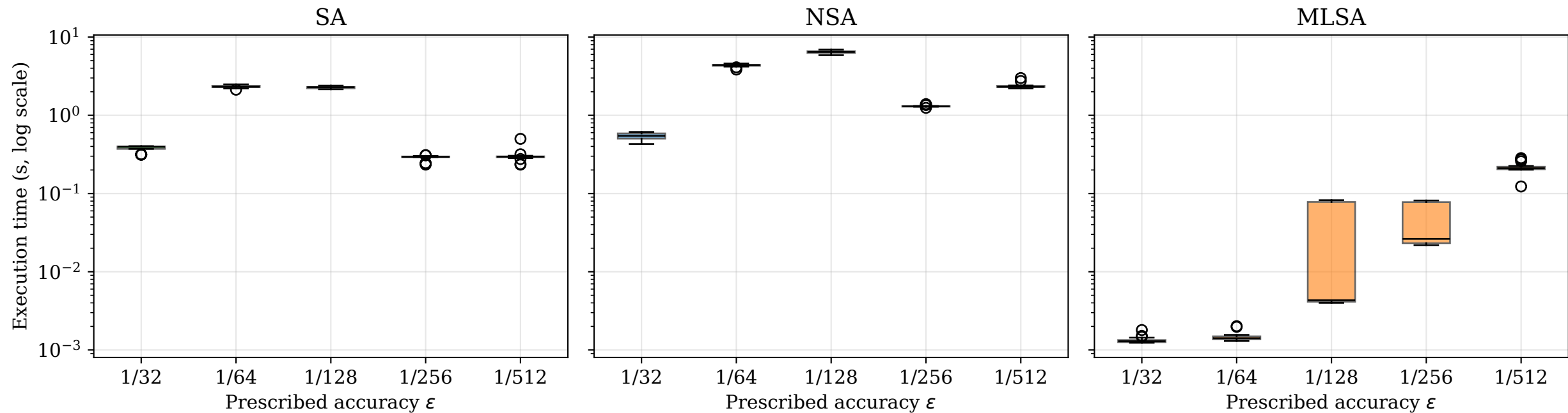
Bs VaR: distribution of execution times across 200 replications
