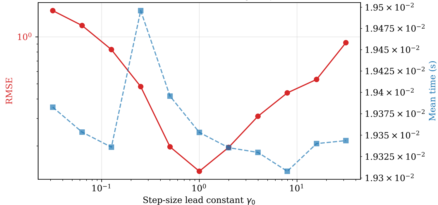
bs VaR: MLSA sensitivity to \gamma_0
