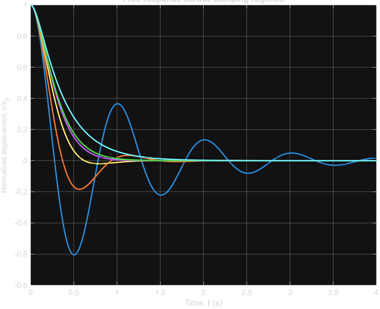
Free response across damping regimes
