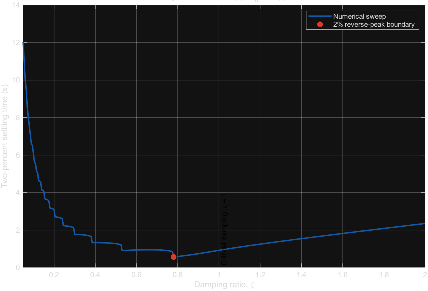
Settling-time tradeoff for x(0) = x_0 and v(0) = 0
