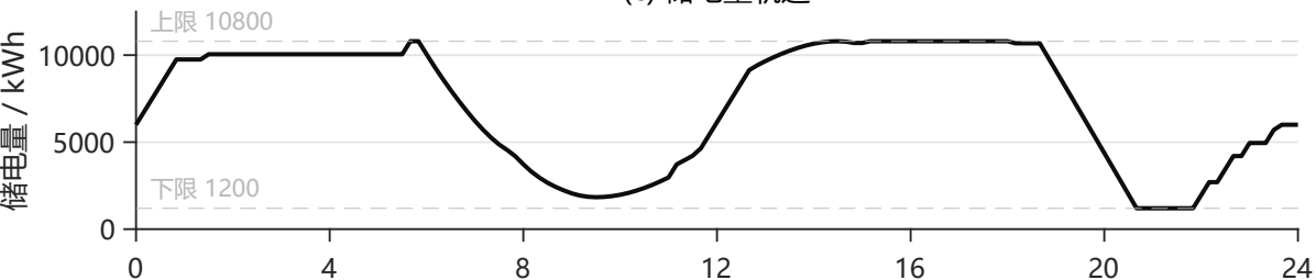
(c) 储电量轨迹
