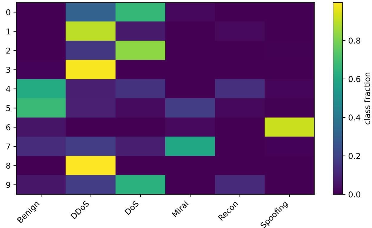
Non-IID class distribution across simulated farm gateways
