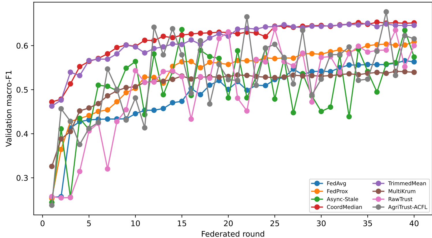
Federated convergence under heterogeneous clients
