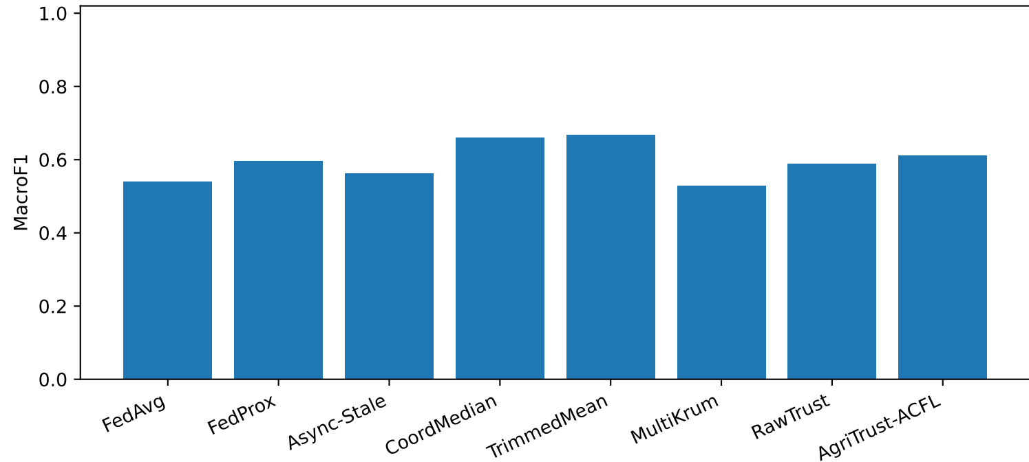
Test MacroF1 comparison
