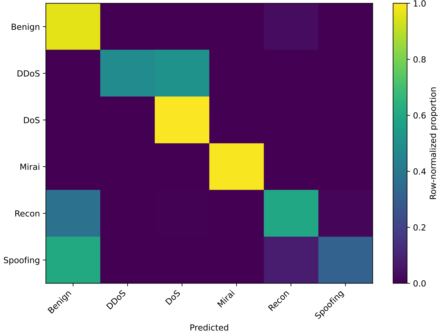
Normalized confusion matrix — TrimmedMean
