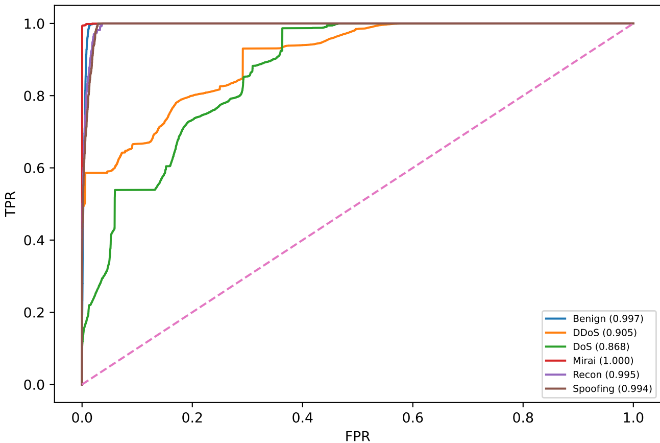
Class-wise ROC — TrimmedMean
