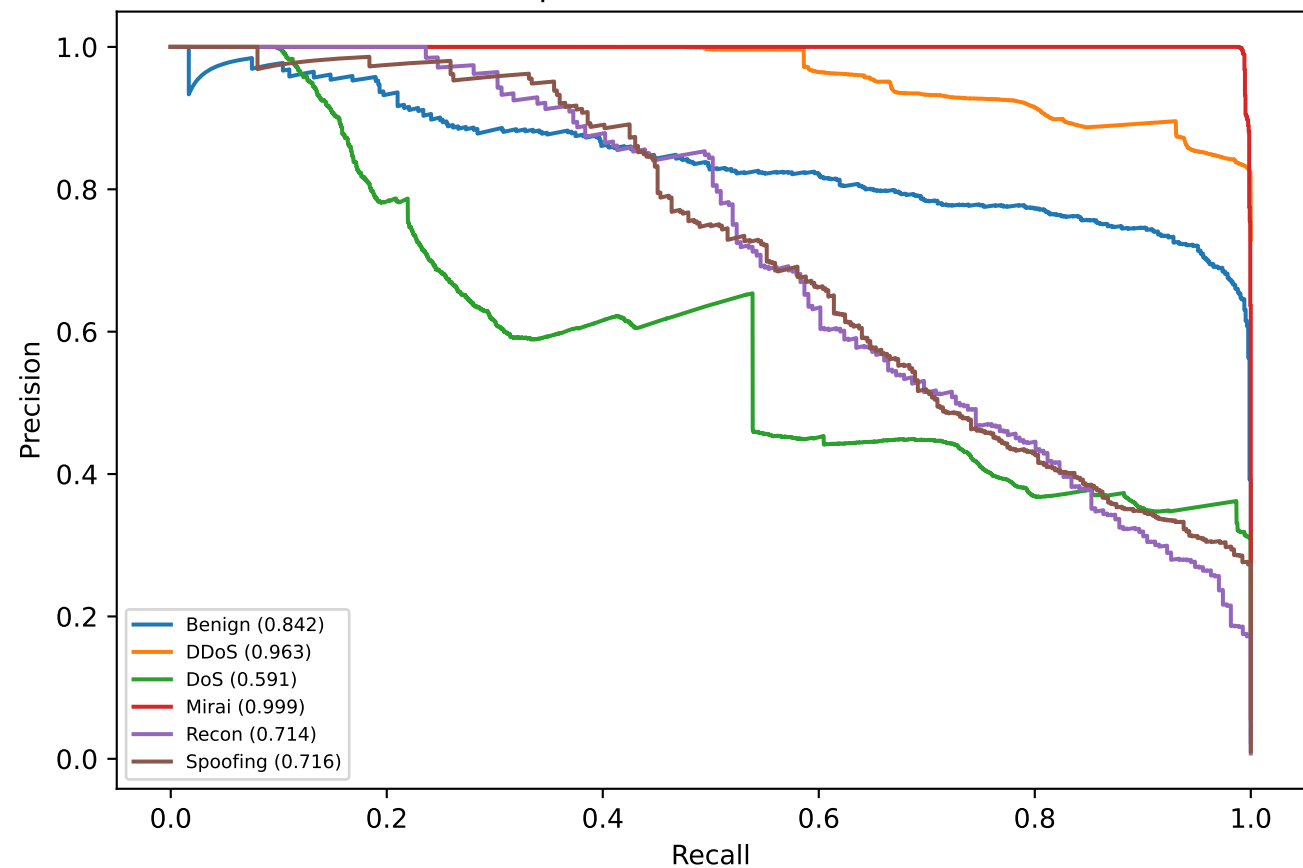
Class-wise precision-recall — TrimmedMean
