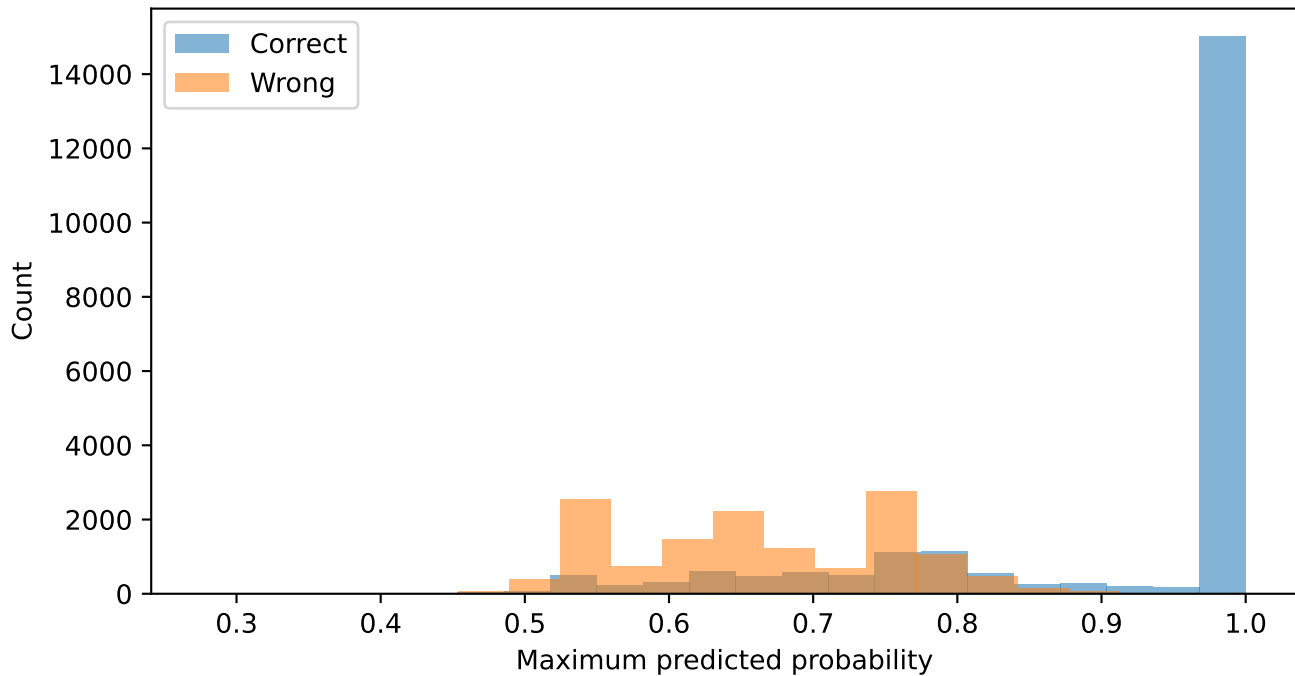
Prediction confidence audit — TrimmedMean
