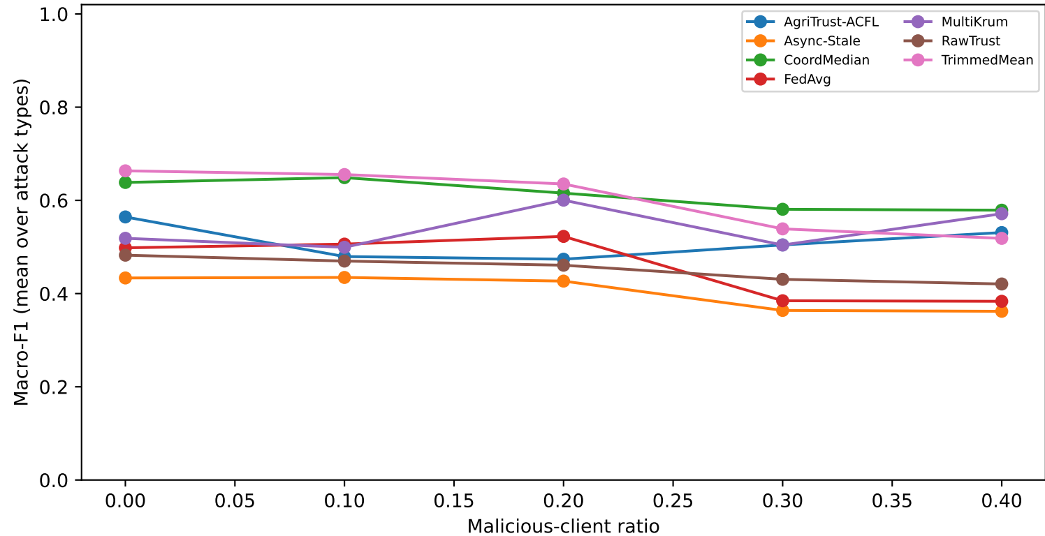
Poisoning robustness across malicious-client ratios
