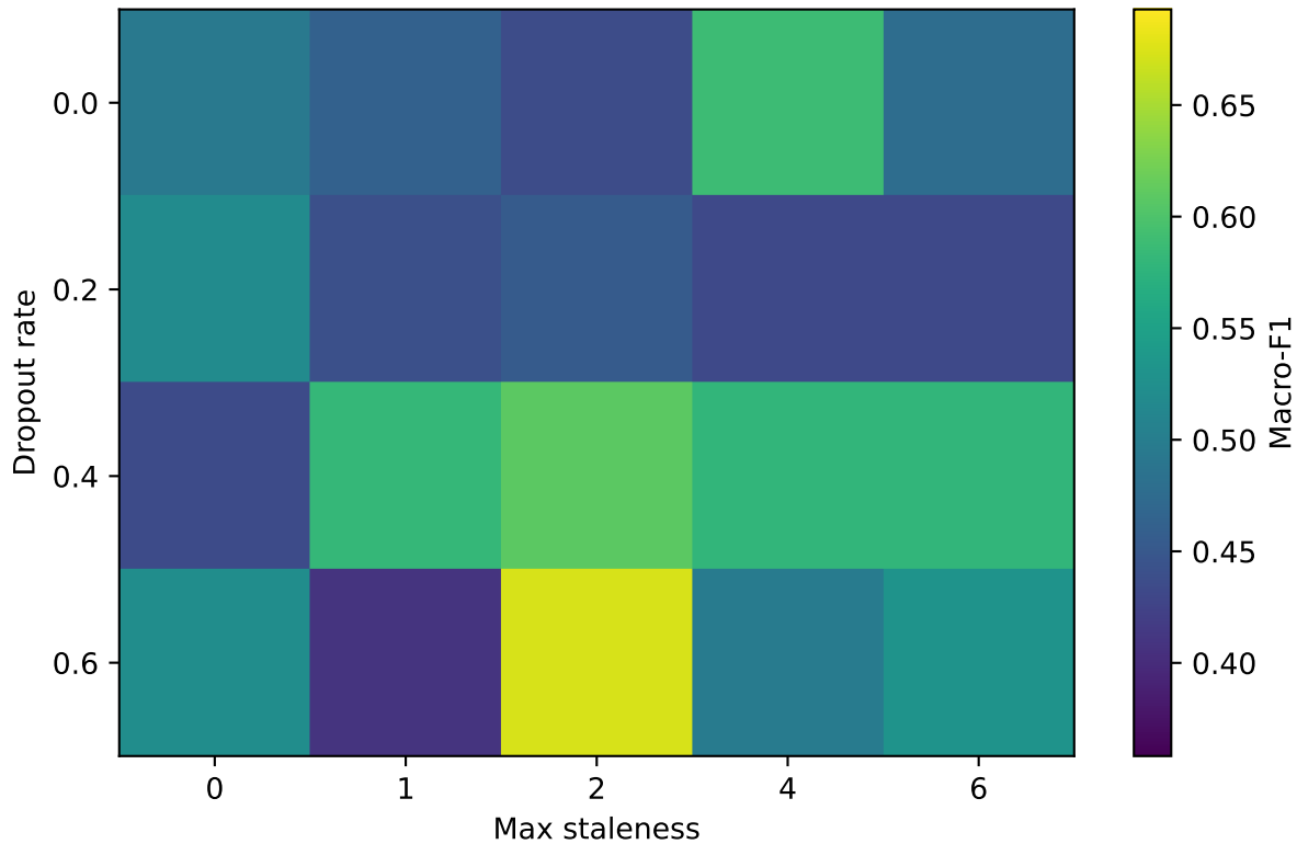
Async-Stale: connectivity robustness
