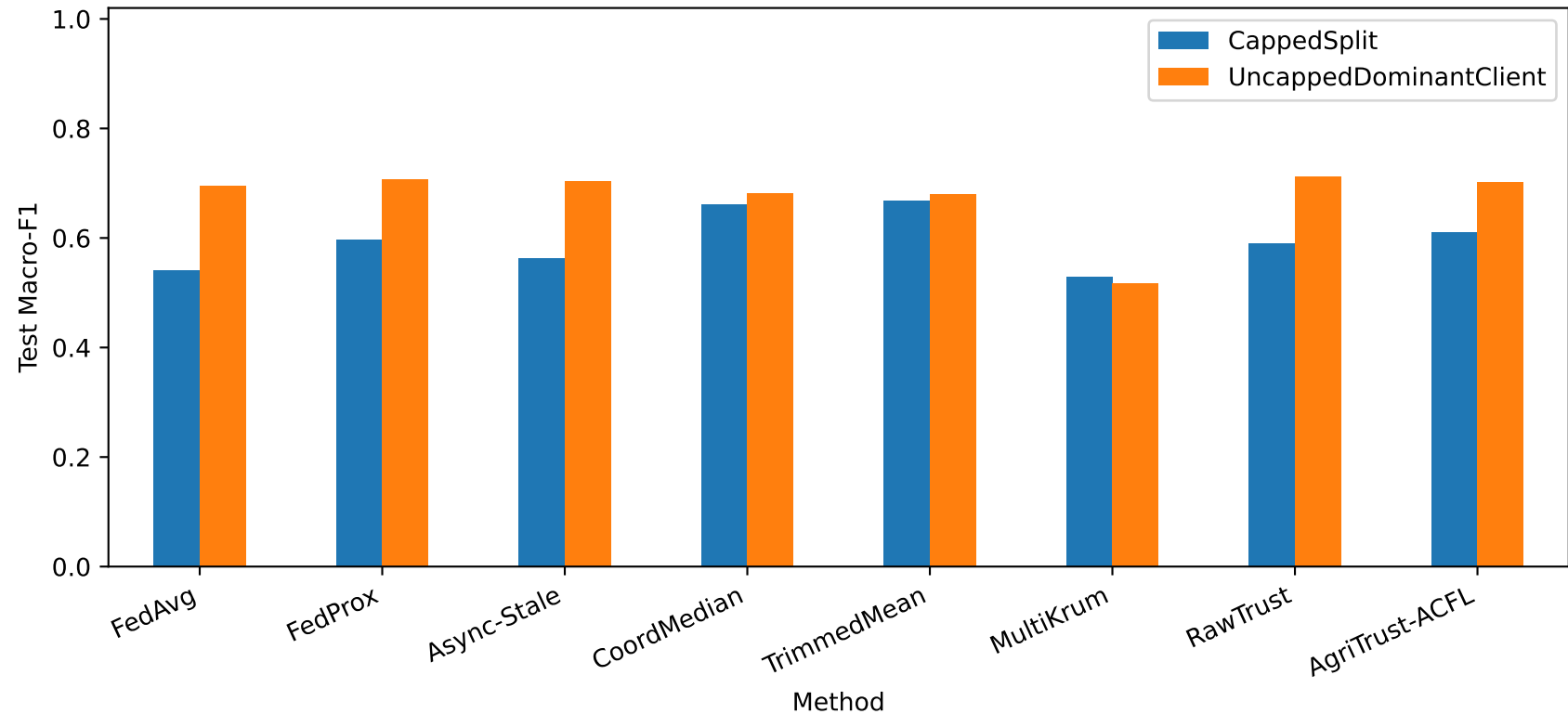
Capped split vs dominant-client split
