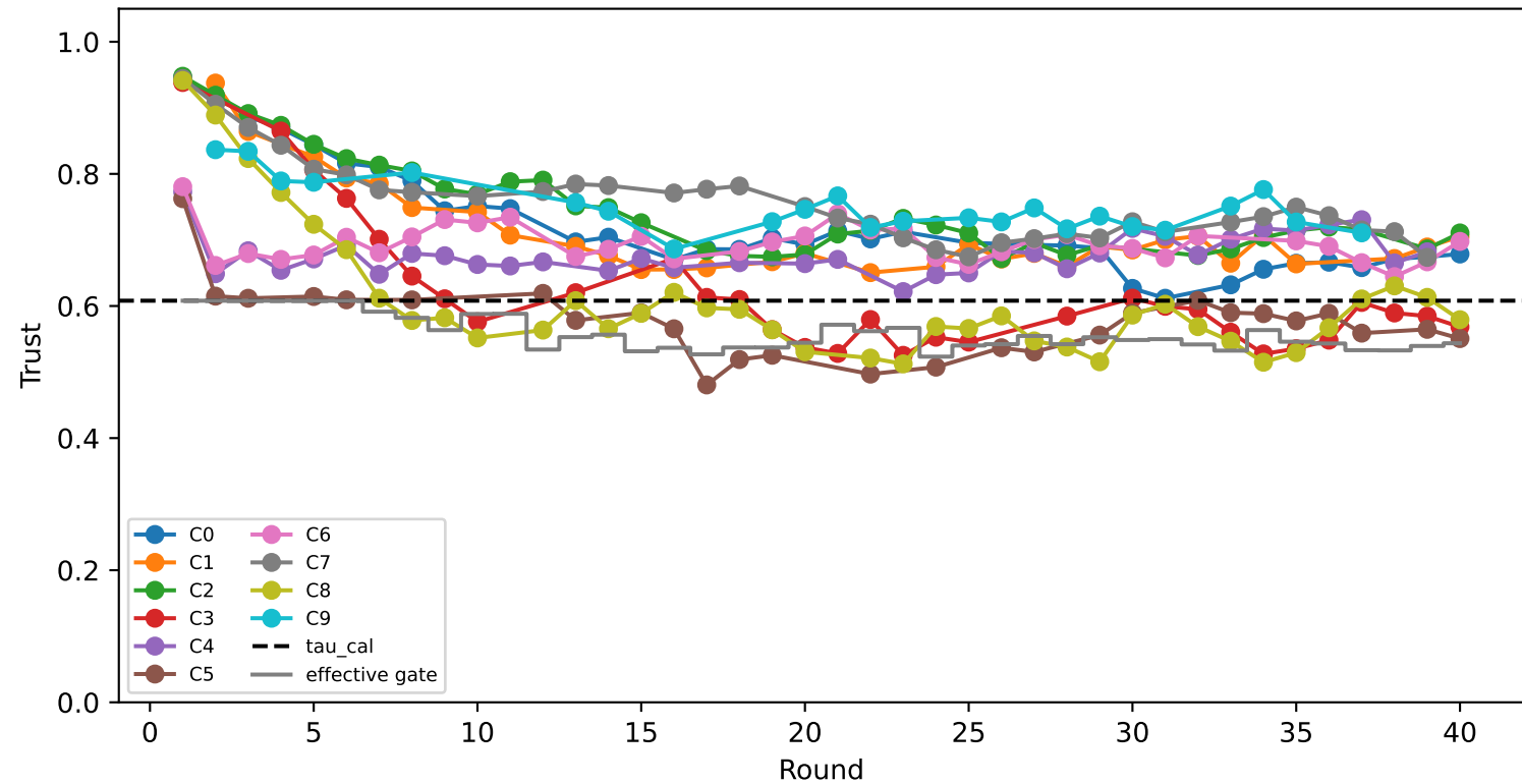
Client trust trajectory during clean federation
