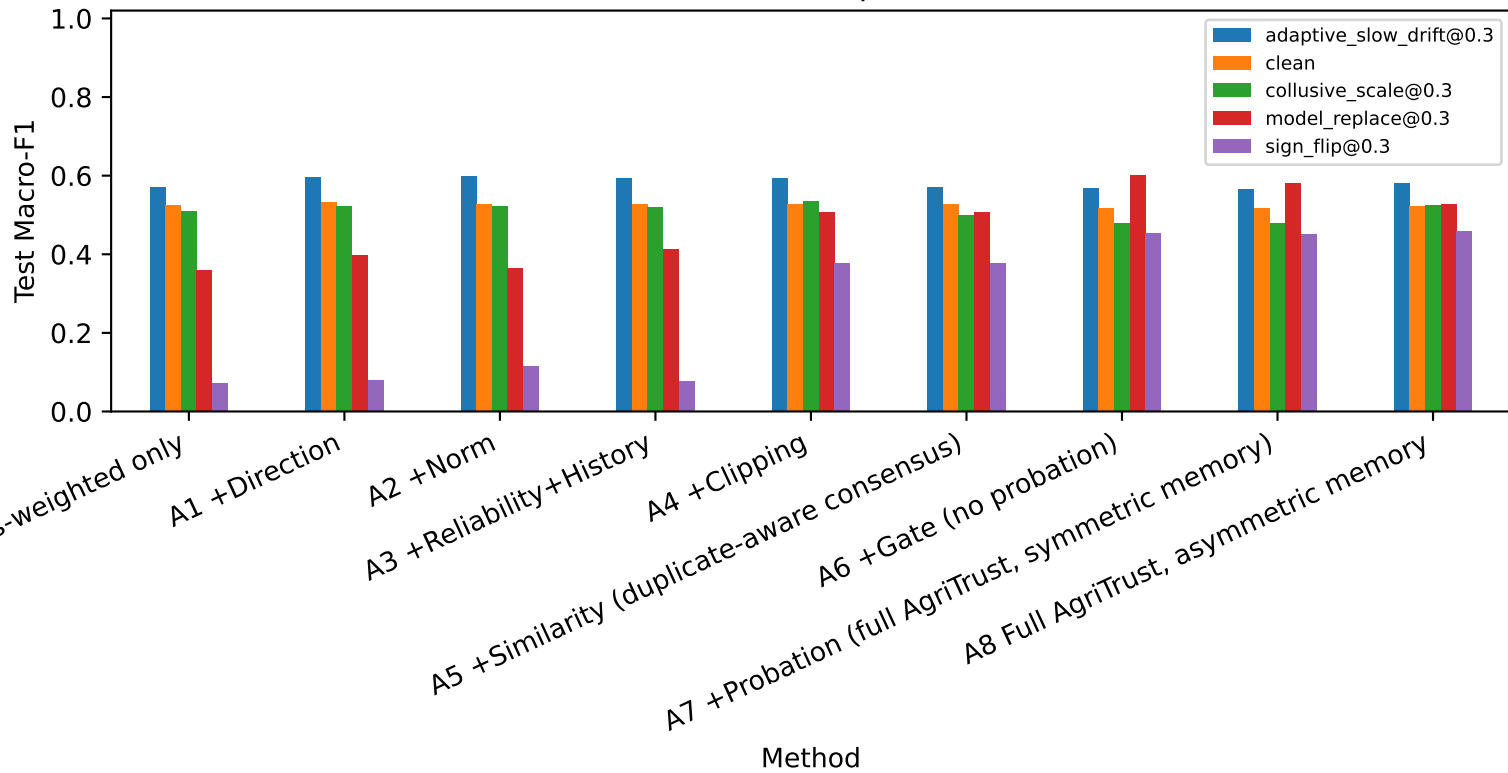
Cumulative trust-component ablation
