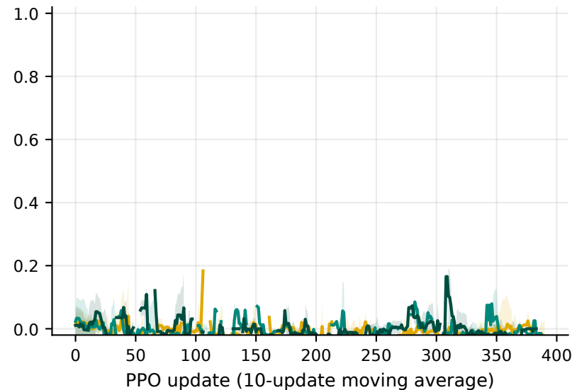
partner-defense rate
