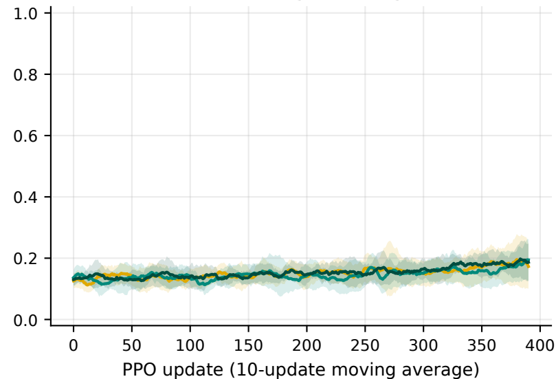
same-target voting
