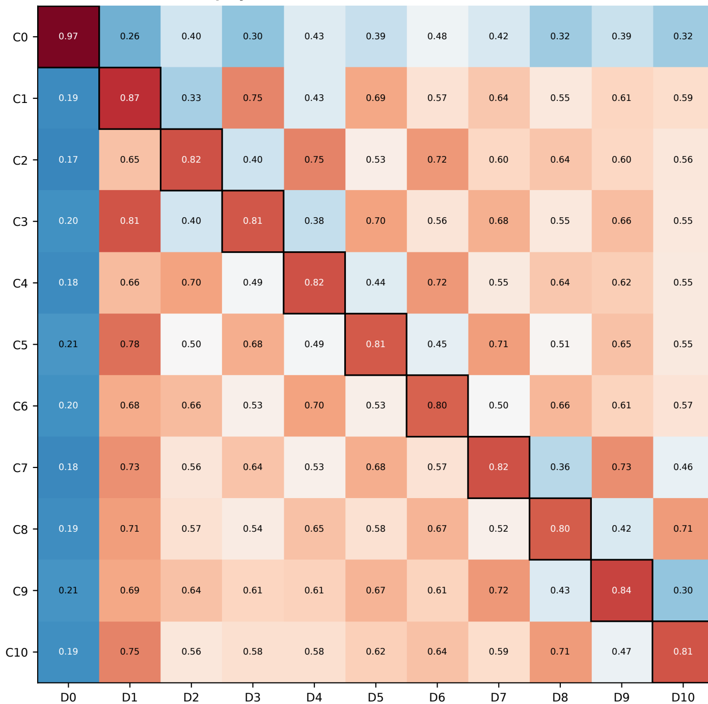
5+2 players, multi-round game cross-play, mean of 10 seeds; boxes = C_i vs its own D_i
