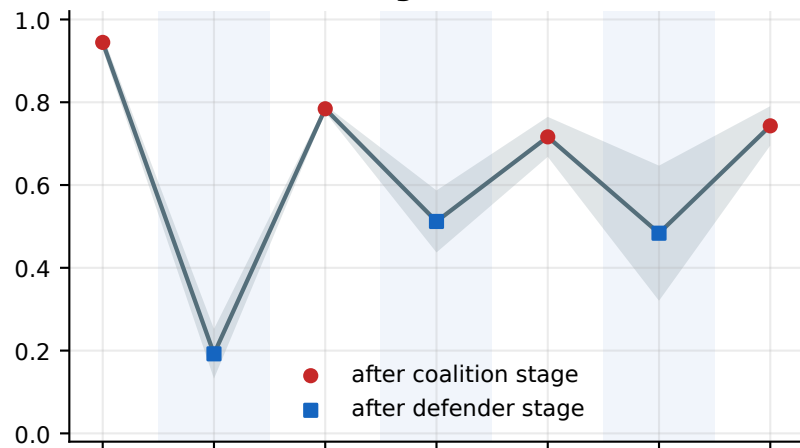
same-target voting
