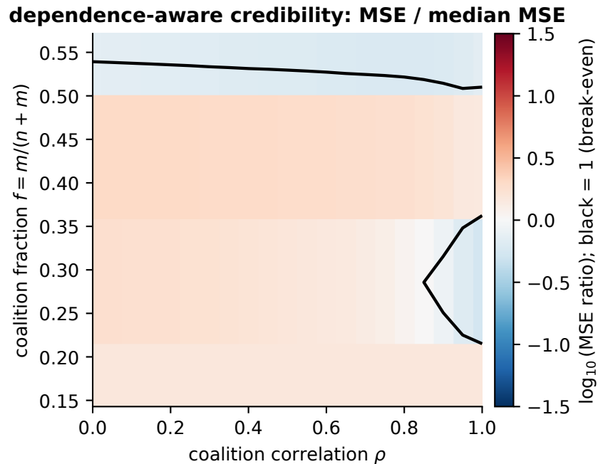
Gaussian report aggregation: simulated MSE and surrogate weight N = 7, \gamma = 1.0, b = 4.0\sigma, h = 0.4\sigma, T = 8, \lambda = 4.0 ; red = larger MSE than the median
