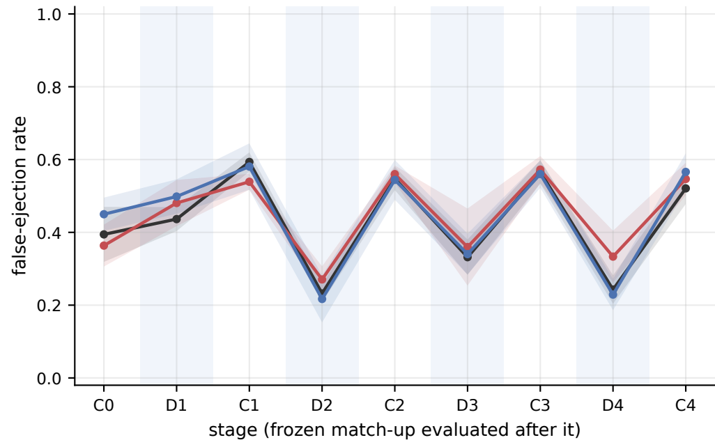
reward specification control, 5+2 single meeting (mean \pm SD across seeds)
