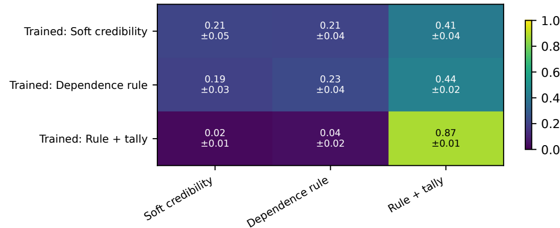
Single-meeting false ejection
