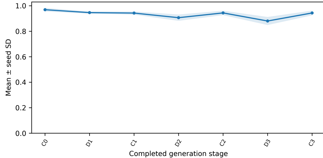
Coalition game wins
