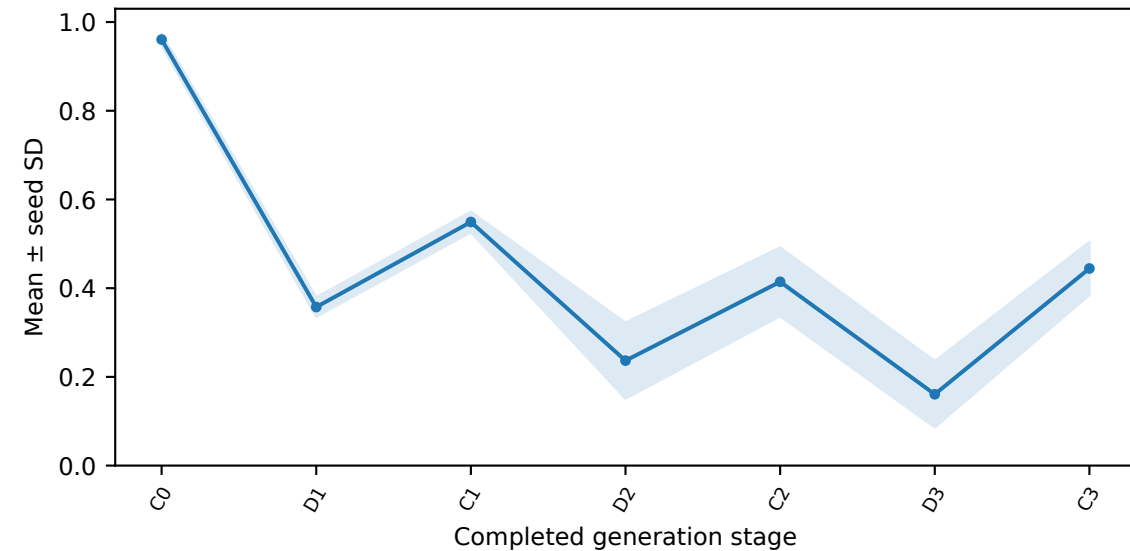
Terminal-meeting false ejection
