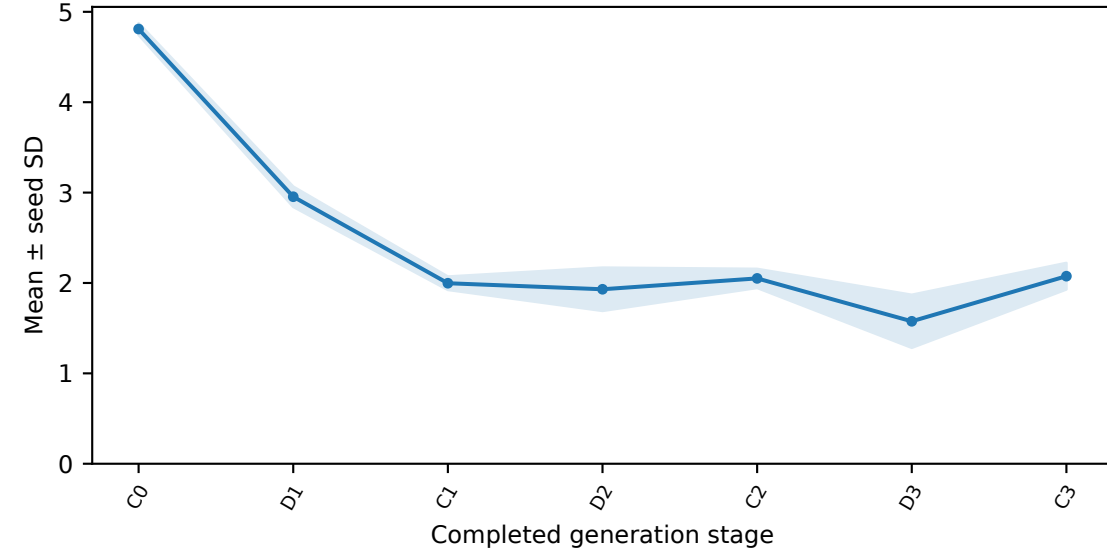
Terminal-meeting false ejection
