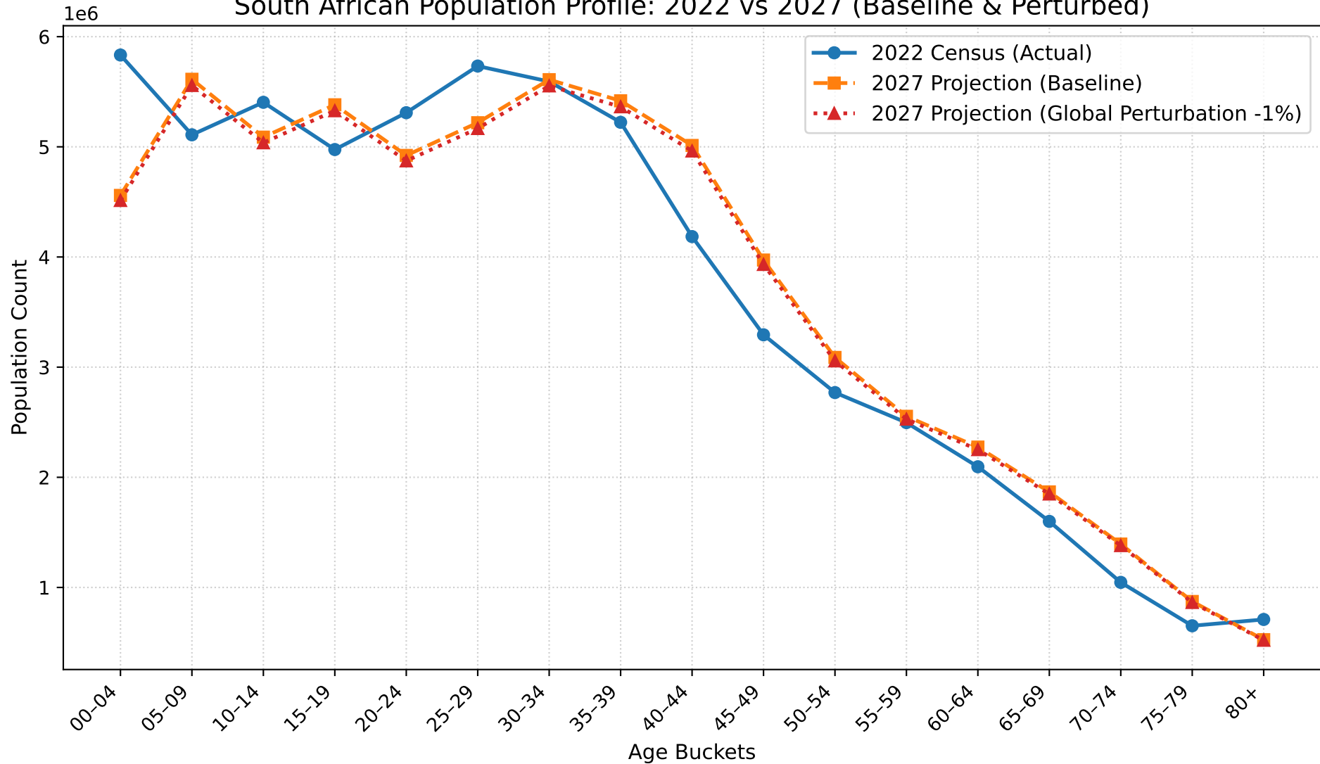
South African Population Profile: 2022 vs 2027 (Baseline & Perturbed)
