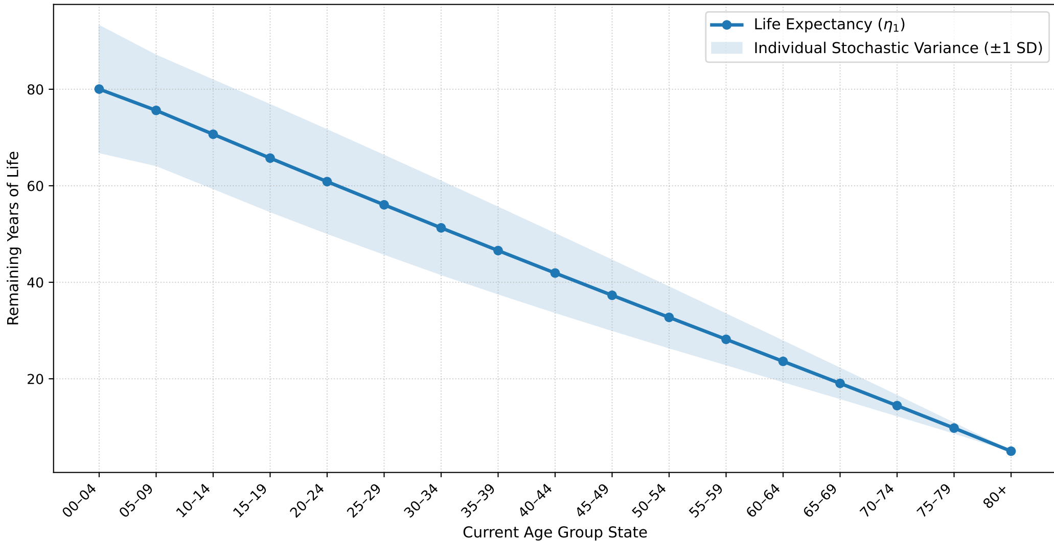
Corrected Stochastic Longevity: South African Life Expectancy & Variance
