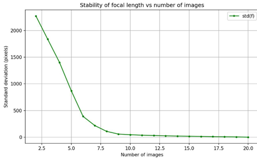
Figure 5: standard deviation of focal length as a function of number of images
