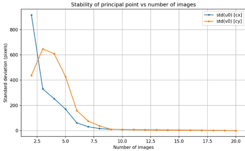
Figure 4: standard deviation of u_0 and v_0 as a function of number of images
