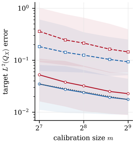
(b) Exact weighted, pinball MLP n = 8192
