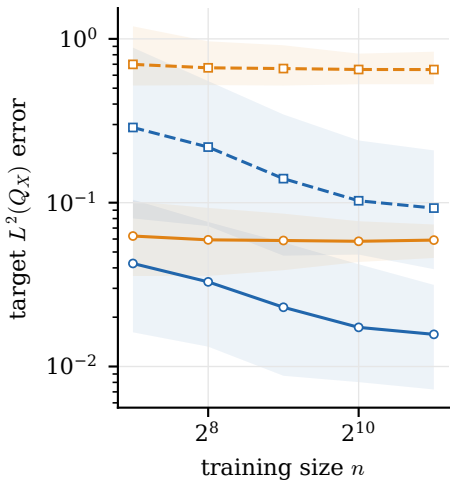
(c) Training-size effect m = 4096, \kappa = 3
