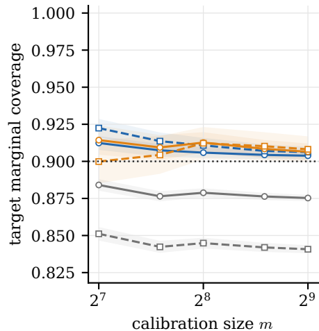
(a) Validity, linear QR n = 2048
